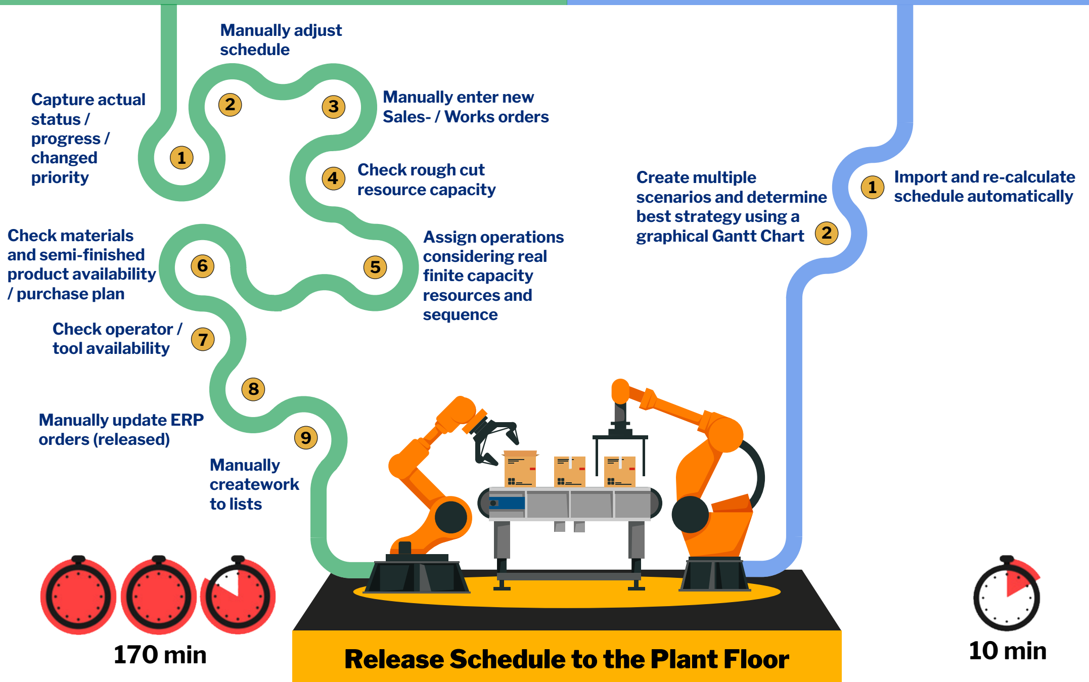
Opcenter Scheduling
