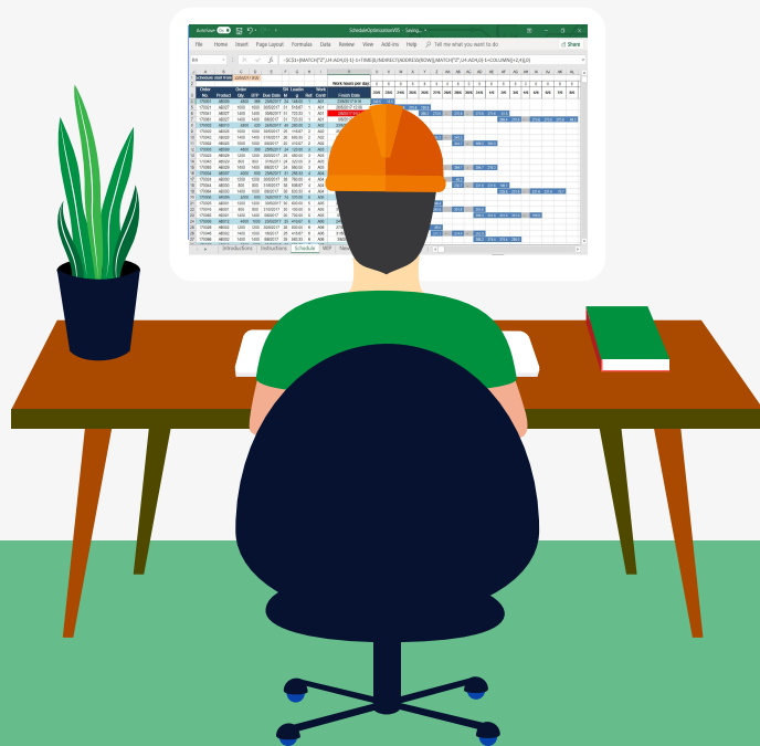
Excel Based
