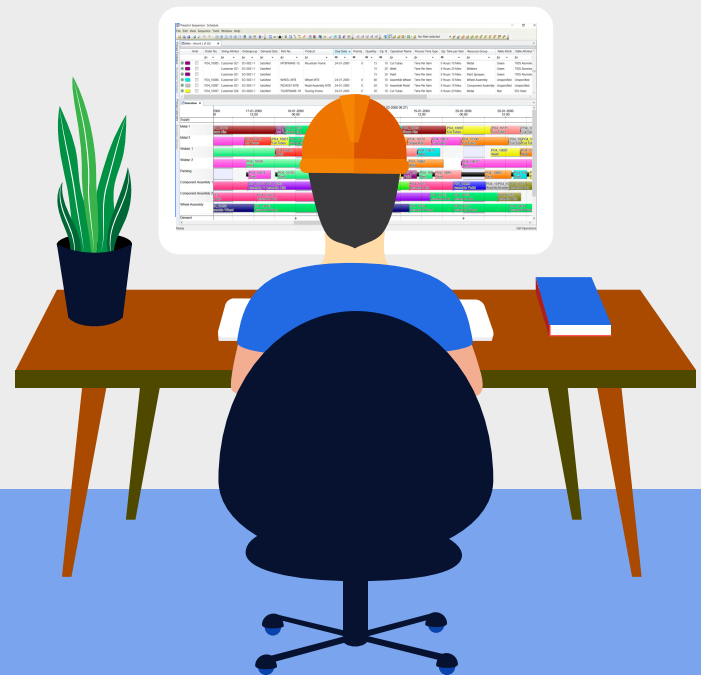
Opcenter Scheduling
